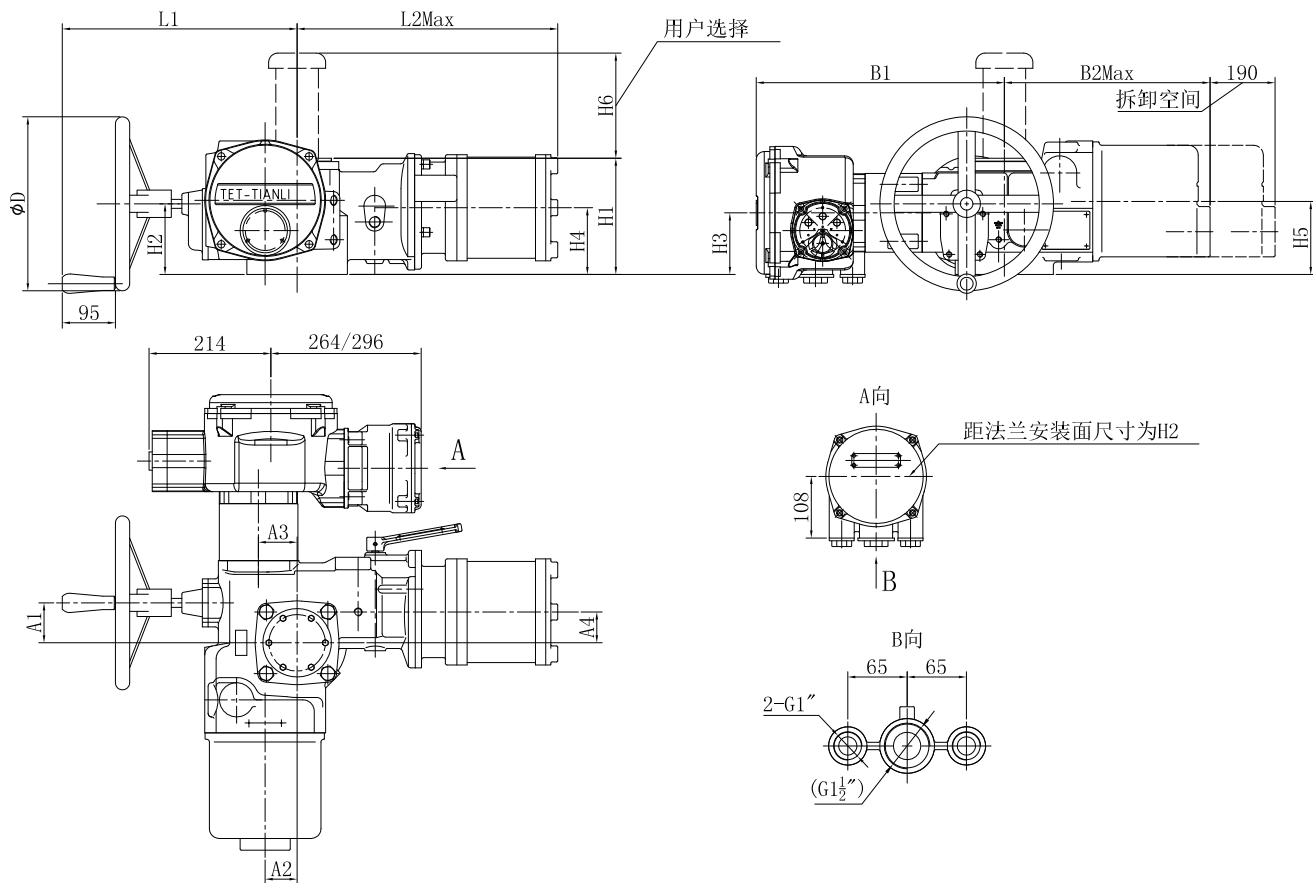
SMC-00~2防爆型、整体防爆型外形尺寸
